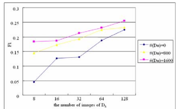
Figure 5: The performances of our method with different number of labeled images and with different number of unlabeled images.
