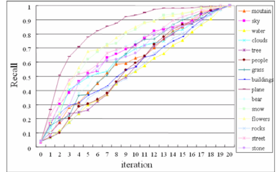
(a). recalls for each of 15 labels.
